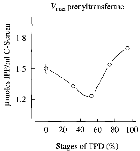
Figure 2 B. V_{max} of prenyltransferase in the C-serum of latex harvested from trees at different stages of tapping panel dryness.
