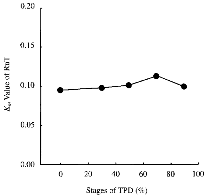
Figure 1 B. K m value of rubber transferase in the latex harvested from trees at different stages of tapping panel dryness.
