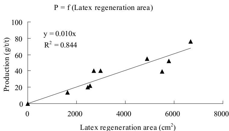
Figure 4. Multi-clonal linear regression between rubber production (the last month before latex sampling), expressed in g/t/t, and the estimated latex regeneration area, expressed in cm 2 .
