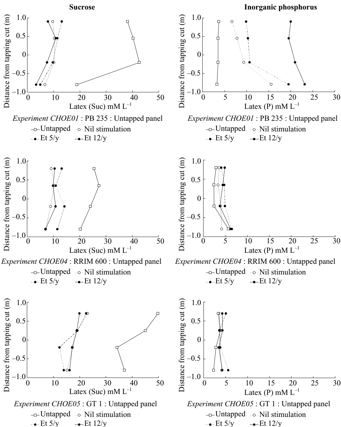
Figure 2. Vertical distribution of latex sucrose content [(Suc), \text{mM L}^{-1} ] and latex inorganic phosphorus content [(P), \text{mM L}^{-1} ] on the untapped panel of clones PB 235, RRIM 600 and GT 1, depending on the distance from the tapping cut ( \pm 90 cm). Sampling was carried out at four positions, equivalent to the following positions on the tapped panel: 20 cm and 80 cm below the cut, 10 cm and 55 cm above renewed bark.
